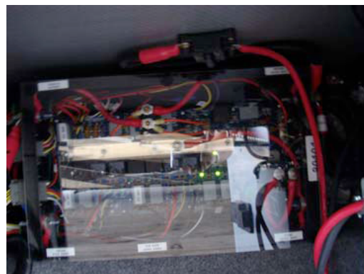
Figure 7-10. Resettable Circuit Breakers
