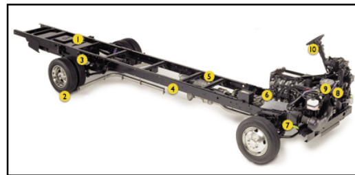
Figure 6-1. Chassis
